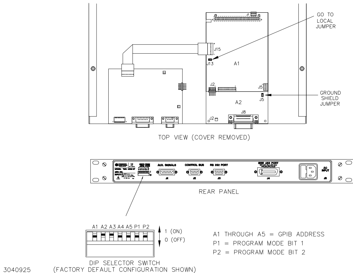
FIGURE 2-1. TMA 4882-27 CONFIGURATION CONTROLS
